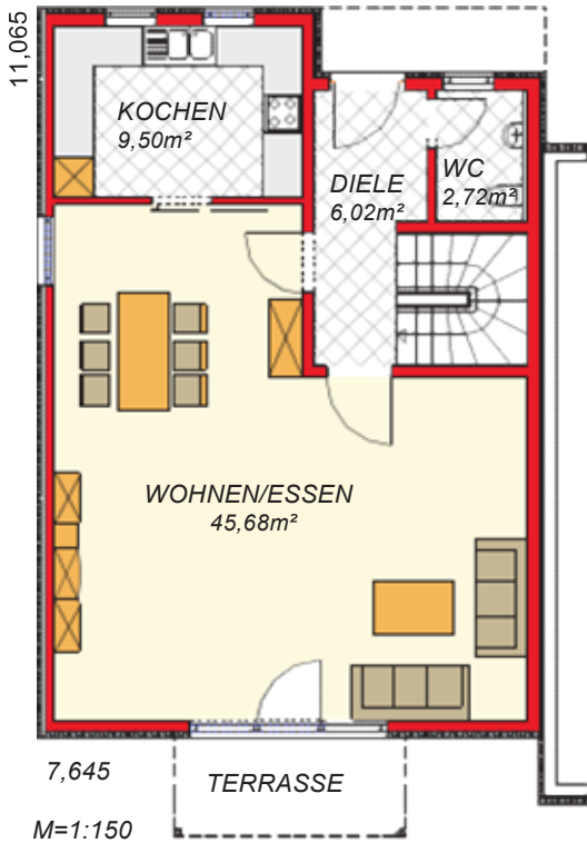
Erdgeschoss VARIANTE A
